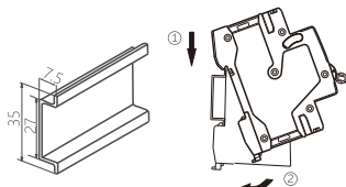
Installation Diagram
