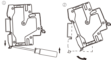
Disassembly Illustration
